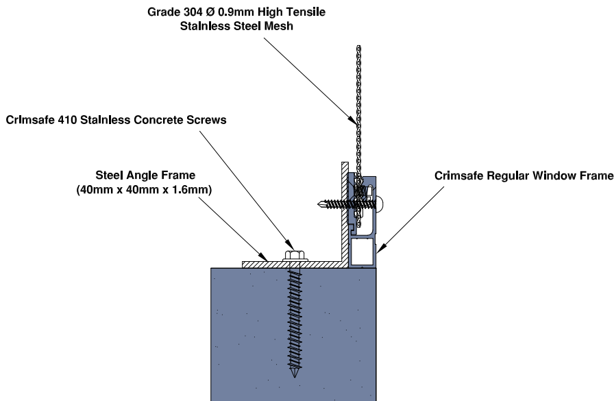
Figure 2 - Reveal fixed to Masonry or Concrete Walls with Steel Angles
