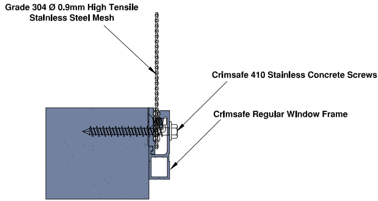
Figure 1 - Reveal fixed to Masonry or Concrete Walls
