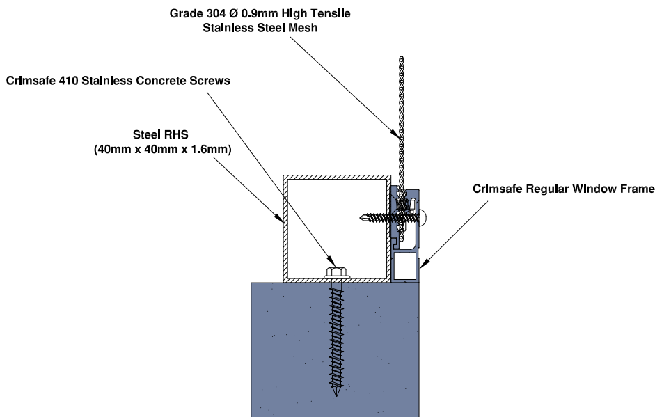
Figure 3 - Reveal fixed to Masonry or Concrete Walls with Steel Tubes
